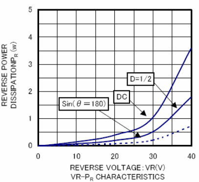
REVERSE VOLTAGE: V_R (V) V_R -P R CHARACTERISTICS
