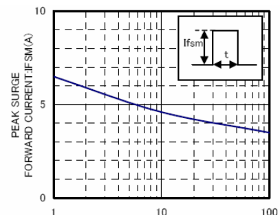
TIME: t (ms) IFSM-t CHARACTERISTICS
