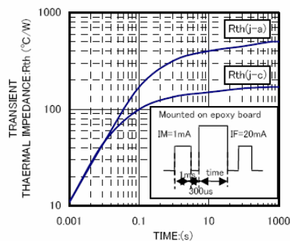
Rth-t CHARACTERISTICS
